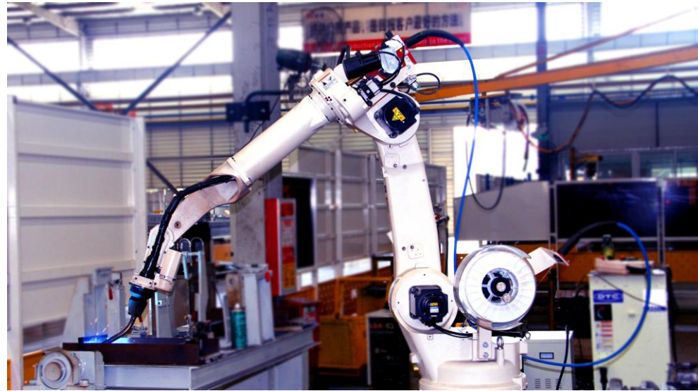
◀ 焊接机器人 A II -B4L A II -B4L welding robot
